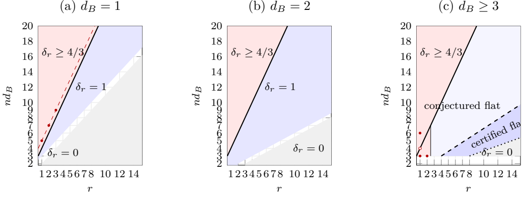
Figure 3: Flat-width regimes of the input-independent body ( d_A = 1 , n d_B > 2 ) in the plane of the latent dimension r and the flag-coordinate count n d_B ; the solid line in every panel is the phase boundary n d_B = 2r + 2 . The drawings are schematic: the regions are exact at the lattice points of each panel within the subcritical range 1 \leq r \leq n d_B^2 - 2 where the classification statements apply (from the affine dimension on, the width is zero, Theorem 5.7); in (a) n d_B = n , in (b) n d_B = 2n , and in (c) n d_B \geq 3 with the dashed and dotted boundaries drawn for d_B = 3 . (a) Classical outputs: \delta_r = 1 between the boundary and the exact-reconstruction region, \delta_r \geq 4/3 above the boundary (Corollaries 6.9 and 6.4); on the dashed line n d_B = 2r + 3 the value is exactly 4/3 (Corollary 6.7), marked at (r, n d_B) = (1, 5), (2, 7), (3, 9) ; the row n d_B = 2 is the collapse case (i) of Theorem 5.18. (b) Qubit outputs: \delta_r = 1 for r \geq n - 1 , equivalently below the boundary, and \delta_r \geq 4/3 above it (Corollary 6.11); the row n d_B = 2 is the collapse case (ii) of Theorem 5.18. (c) Outputs with d_B \geq 3 : \delta_r \geq 4/3 above the boundary (Corollary 6.4) and in the columns r \in \{1, 2\} , where the state-space obstruction applies at every n (Theorems 6.14 and 6.21 with the concentration gate of Lemma 6.24); below the boundary at r \geq 3 , flatness is conjectured (Conjecture 6.26), certified beyond the dashed pinching boundary r = n Q_2(d_B) - 1 (Theorem 5.11; Q_2(3) = 5 by the balanced two-sector split), the strip between the two boundaries being open (Remark 6.25). Filled circles mark instances with value exactly 4/3 : (1, 5) in (a) ( n = 5 ), and in (c) the qutrit at (1, 3) and (2, 3) ( n = 1 ) together with (1, 6) ( n = 2 , where 2(1 - 1/3) = 4/3 , Theorem 6.12); the open circle marks the one-outcome ququart at (1, 4) , where \delta_1 \in [4/3, 3/2] (Corollary 6.23).
