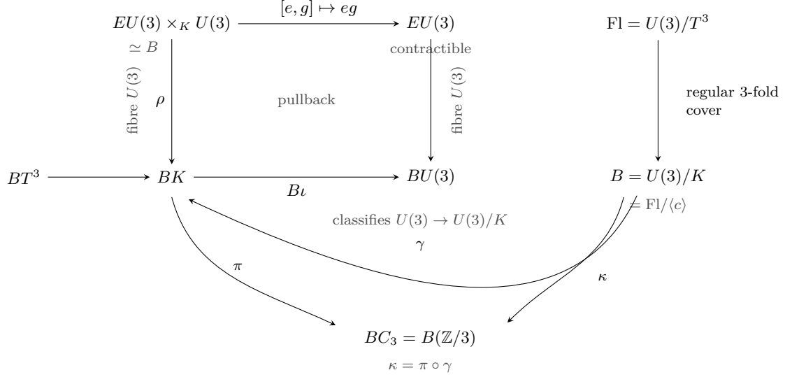
Figure 2: The spaces and maps of the proof of Proposition 6.16. Left: the Borel bundle of Step 1, a fibre bundle with fibre U(3) , total space EU(3) \times_K U(3) homotopy equivalent to B , and base BK ; it is the pullback of the universal bundle U(3) \rightarrow EU(3) \rightarrow BU(3) along B\iota: BK \rightarrow BU(3) , with [e, g] \mapsto eg on top and BK = EC_3 \times_{C_3} BT^3 as in Step 2. Right: the homogeneous models of Step 0, the flag manifold Fl = U(3)/T^3 and the quotient B = U(3)/K = Fl/\langle c \rangle under the regular three-fold cover with deck group \langle c \rangle \cong \mathbb{Z}/3 , together with the classifying maps of Step 6: \gamma classifies the principal K -bundle U(3) \rightarrow U(3)/K , \pi is the quotient BK \rightarrow BC_3 , and \kappa = \pi \circ \gamma classifies the cover. The arrow BT^3 \rightarrow BK is the fibre of the fibration of Step 2. Under the identification of the total space with B , the projection \rho equals \gamma ; the deck transformation c acts by right multiplication by the permutation matrix \sigma , and K = T^3 \rtimes \langle \sigma \rangle (Step 0).
